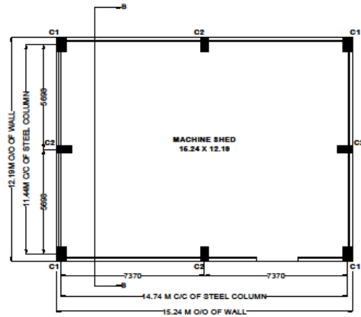
MACHINE SHED
